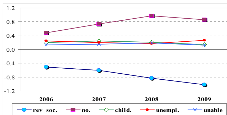
Figure 3.2 Elasticities from the estimated model at the mean values of the variables
